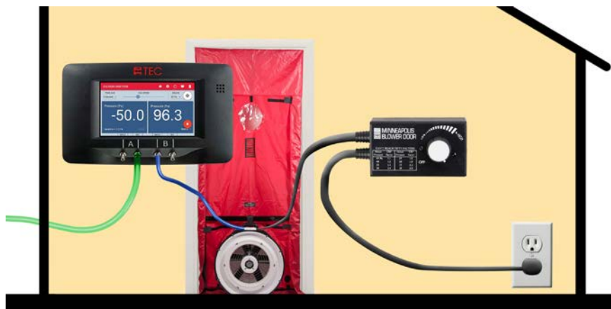
Figure 4. How blower door components are connected.
