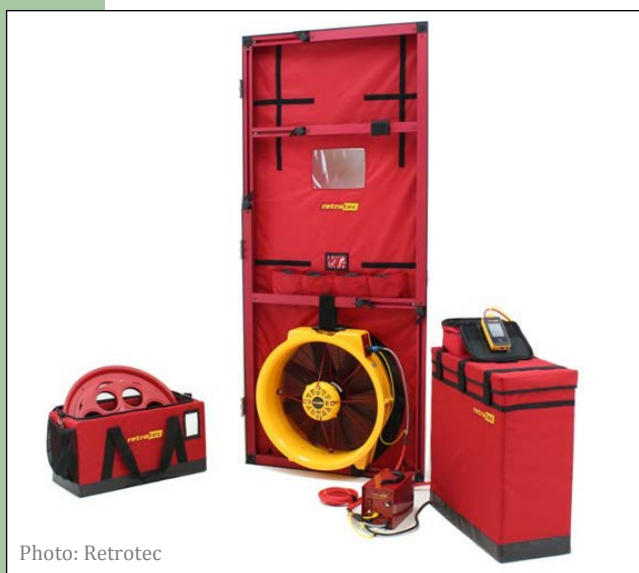
Blower door set up for an air leakage test.
