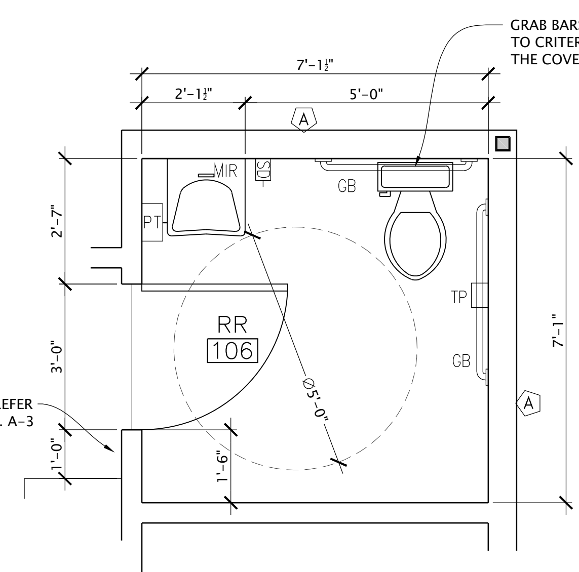
1 ENLARGED PLAN DETAIL SCALE: 1/2" = 1'-0"
