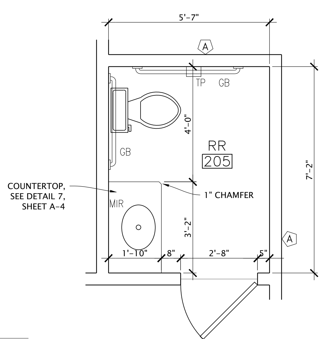
2 ENLARGED PLAN DETAIL SCALE: 1/2" = 1'-0"
