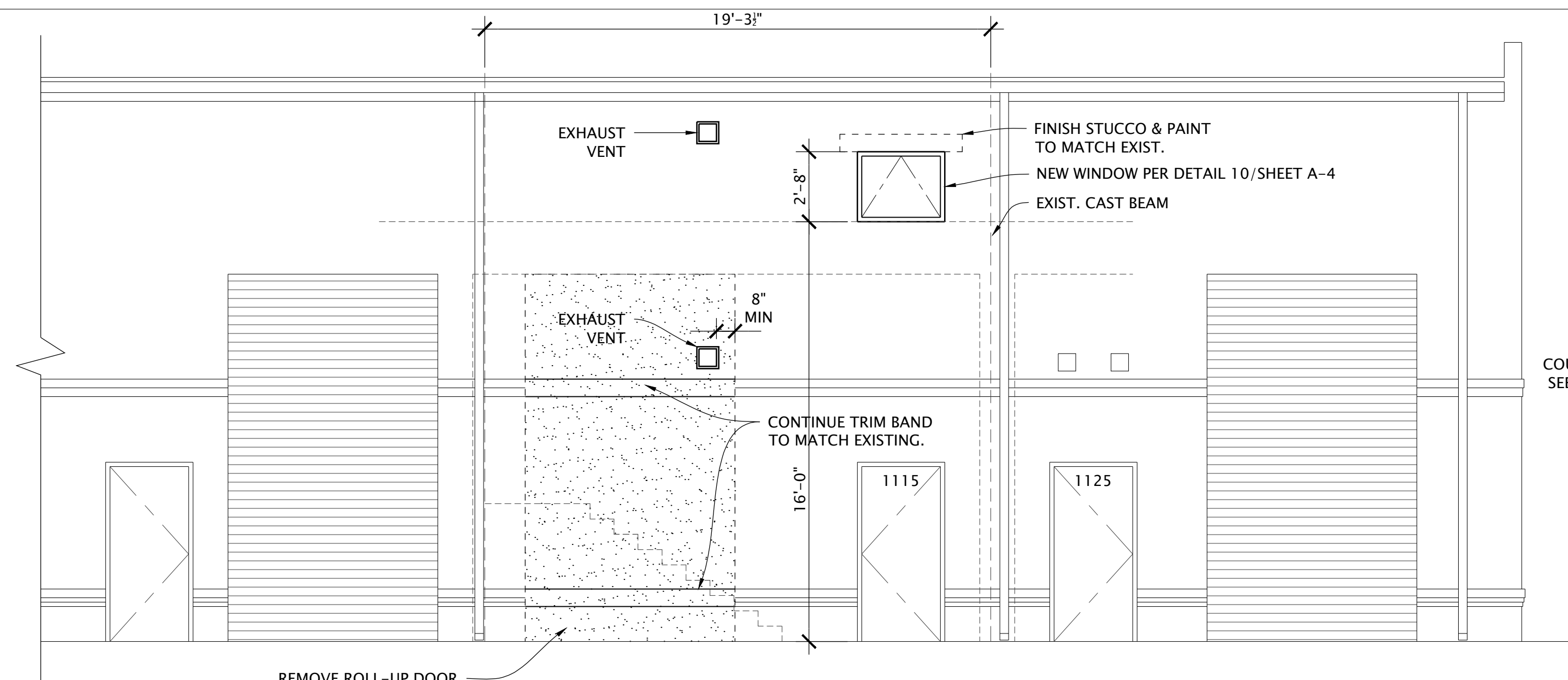
3 NORTH ELEVATION SCALE: 1/4" = 1'-0"
