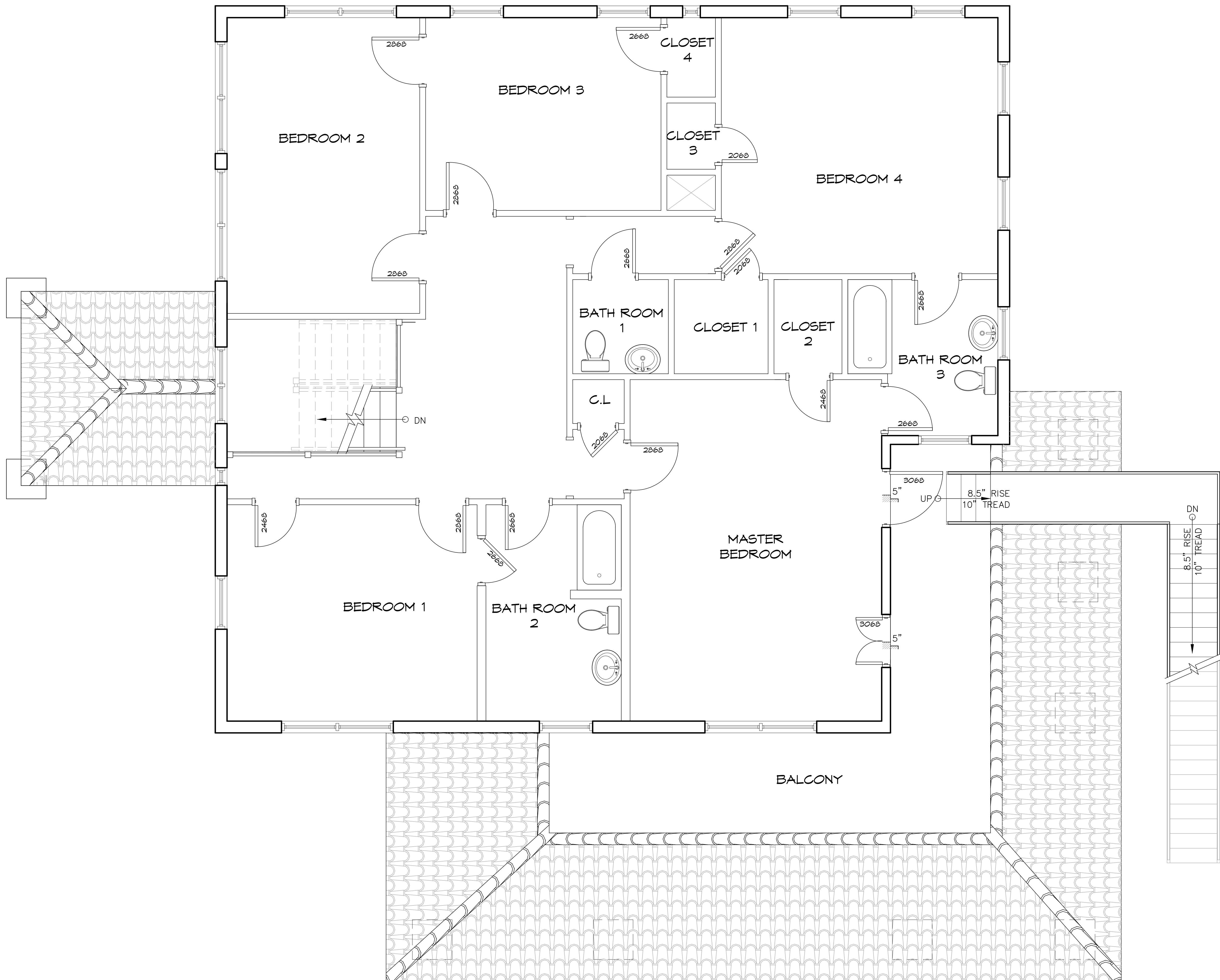
SECOND FLOOR PLAN SCALE: 3/8" = 1'-0"
