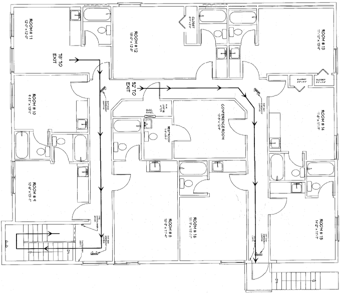
LIFE SAFETY PLAN SCALE 3/16" = 1'-0"
