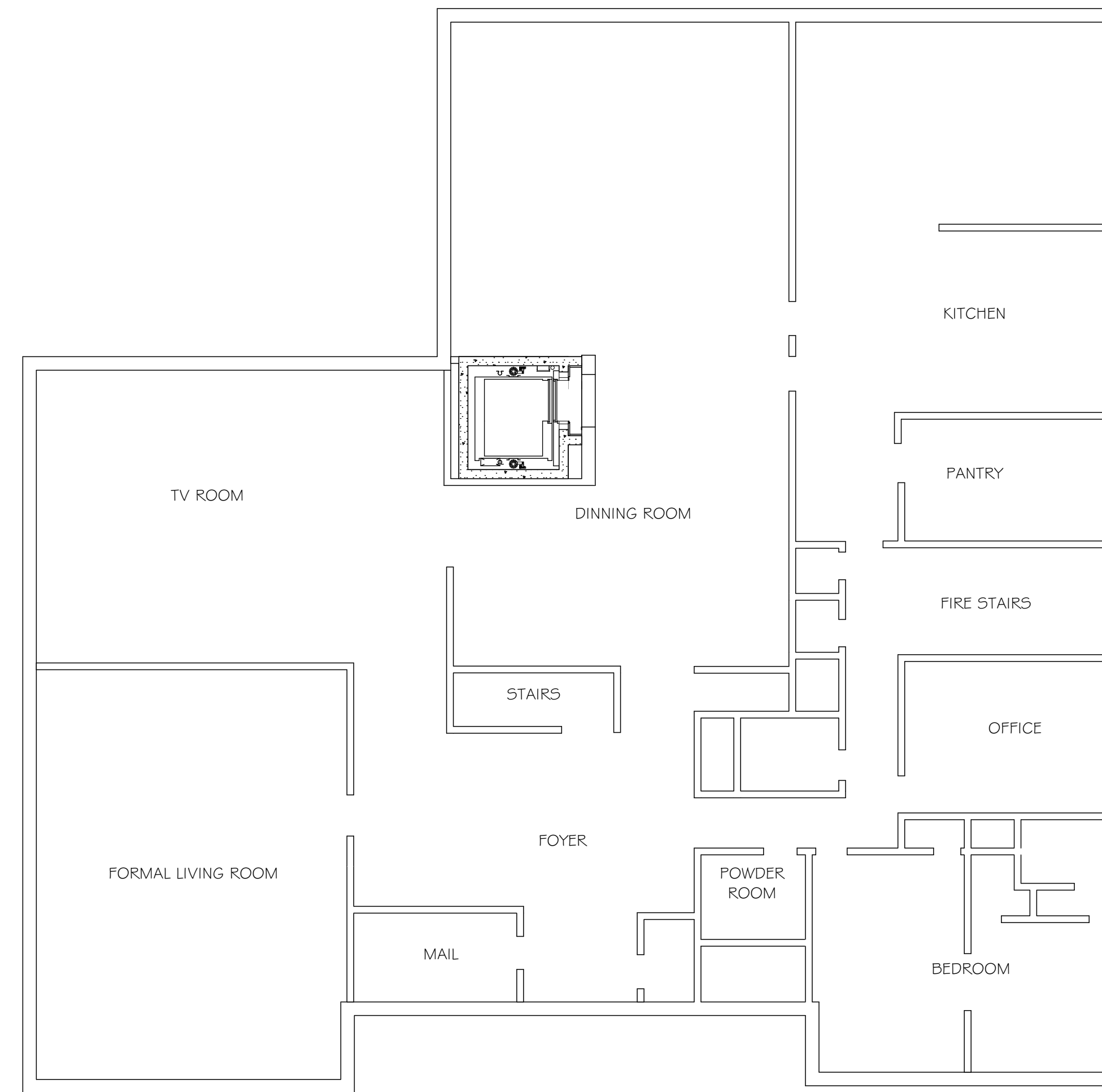
2 ELEVATOR LOCATION @ FIRST FLOOR ASI 1.1 SCALE: 1/8" = 1'-0"
