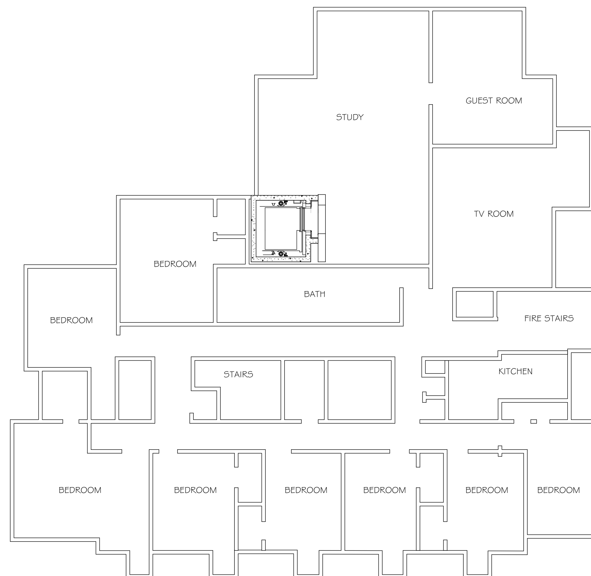
4 ELEVATOR LOCATION @ THIRD FLOOR ASI 1.1 SCALE: 1/8" = 1'-0"
