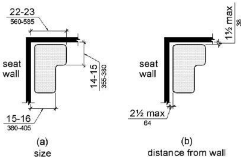
Figure 610.3.2 L-Shaped Shower Seat
