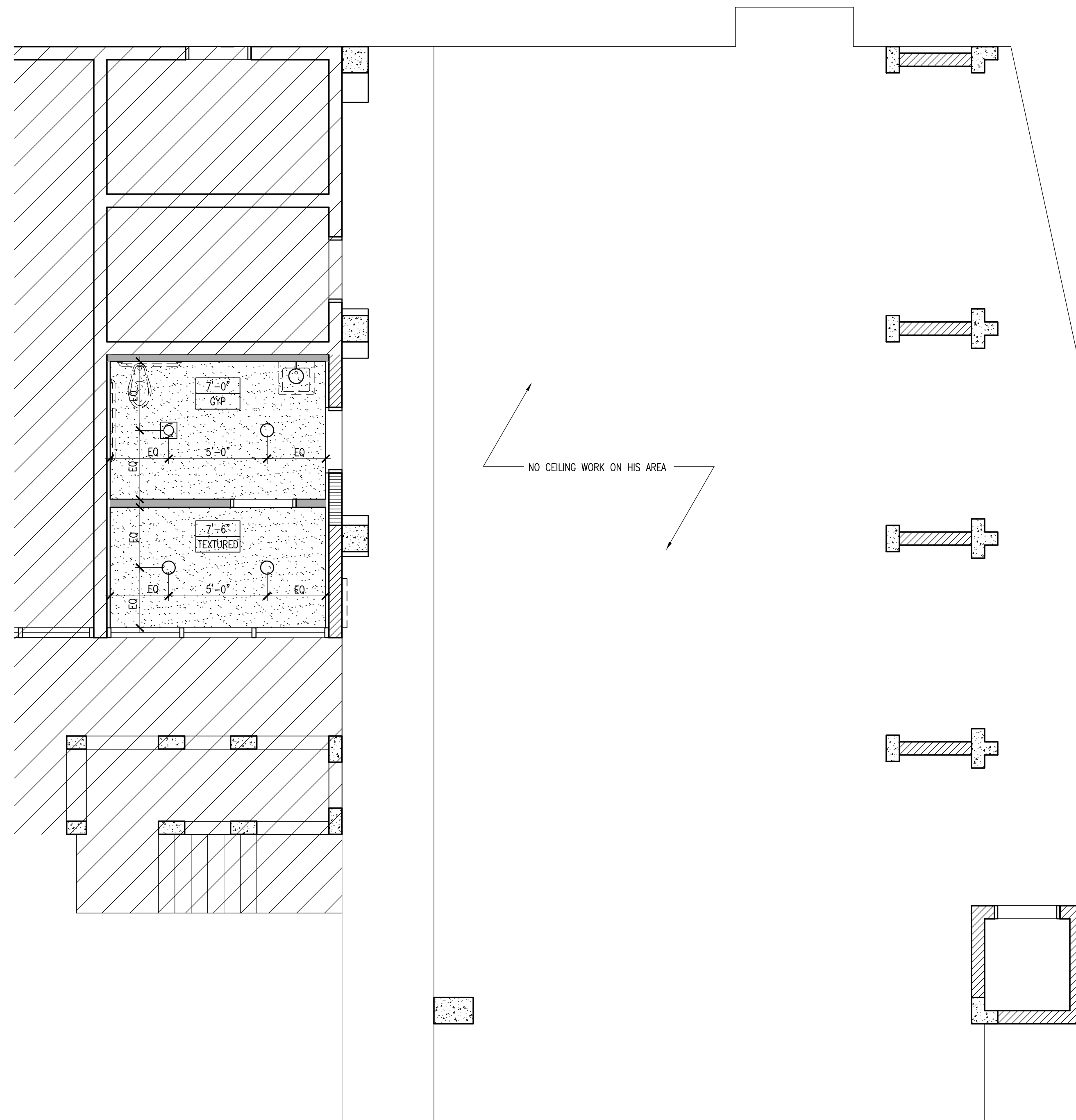
1 FIRST FLOOR REFLECTED CEILING PLAN
