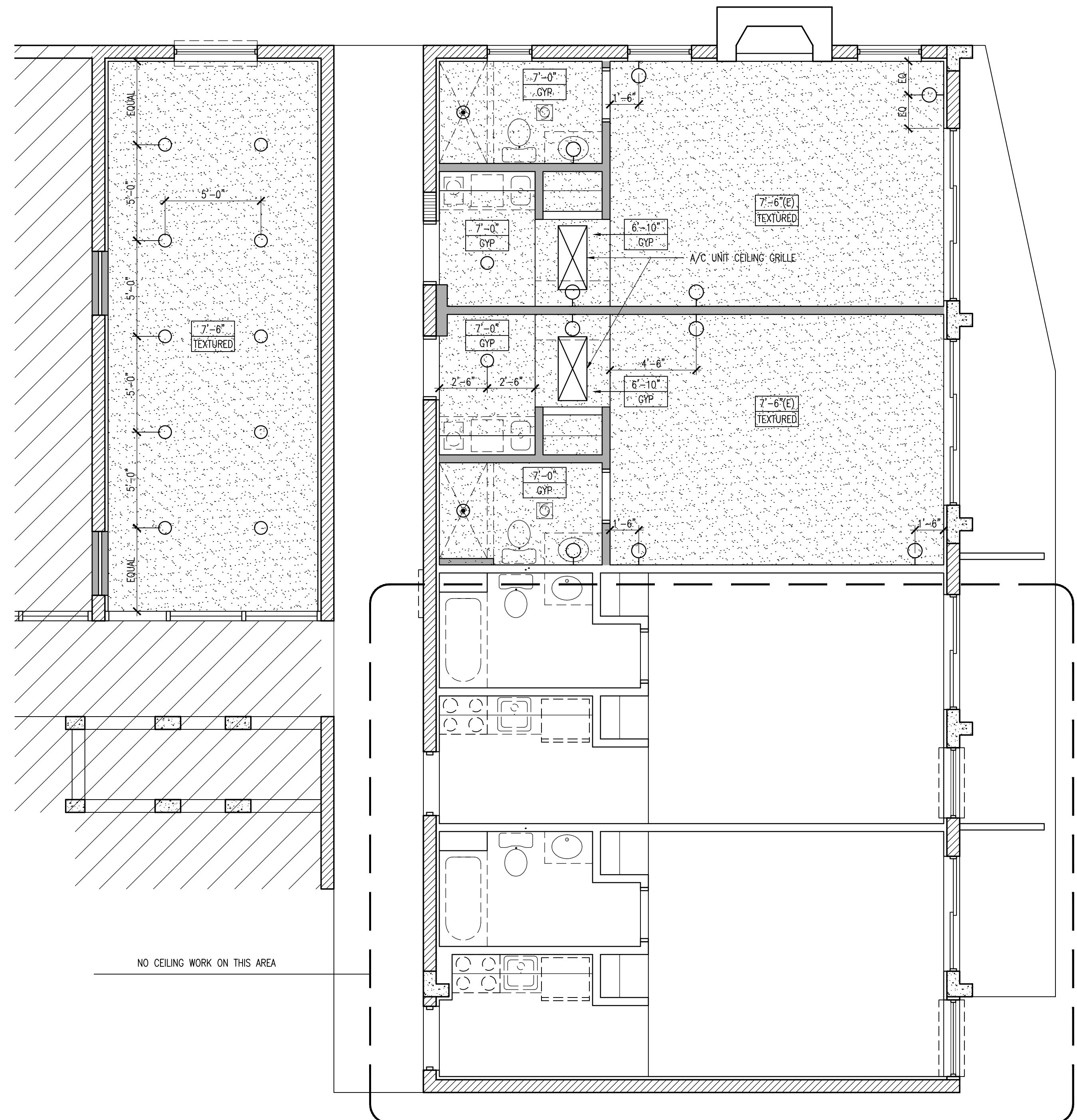
2 SECOND FLOOR REFLECTED CEILING PLAN
