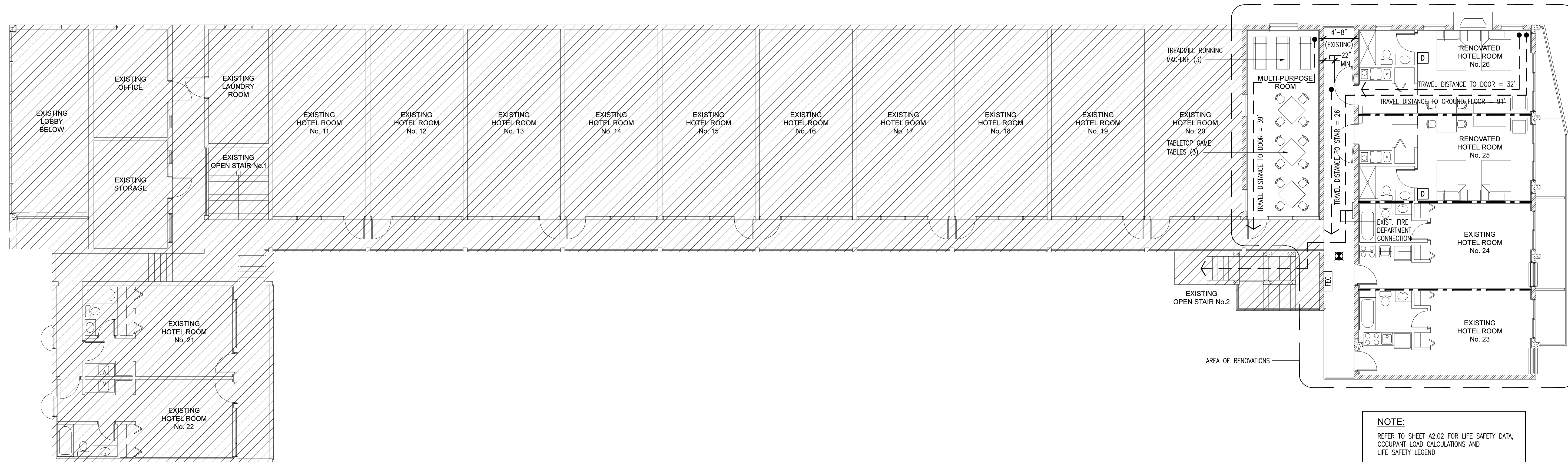
2 SECOND FLOOR LIFE SAFETY PLAN SCALE: 1/8" = 1'-0"
