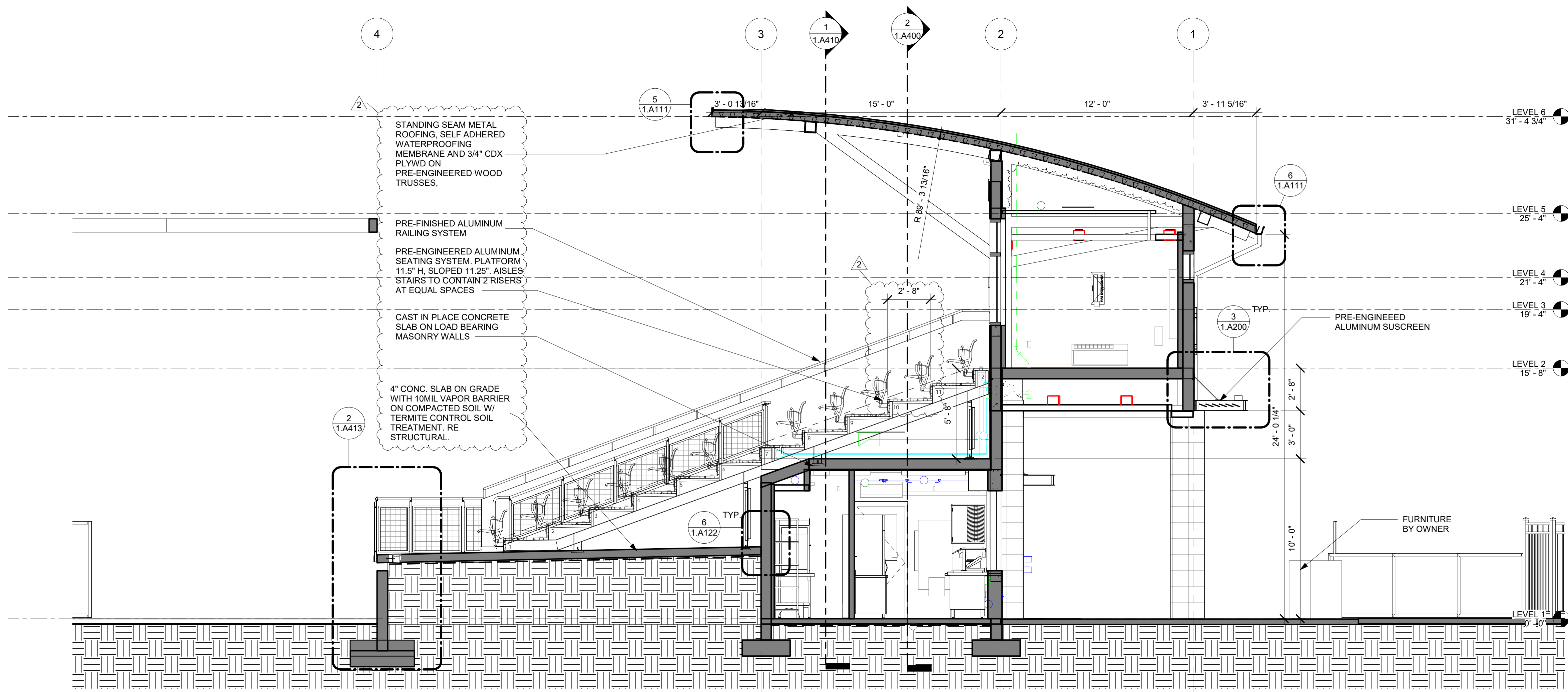
1. BUILDING SECTION 1 1/4" = 1'-0"
