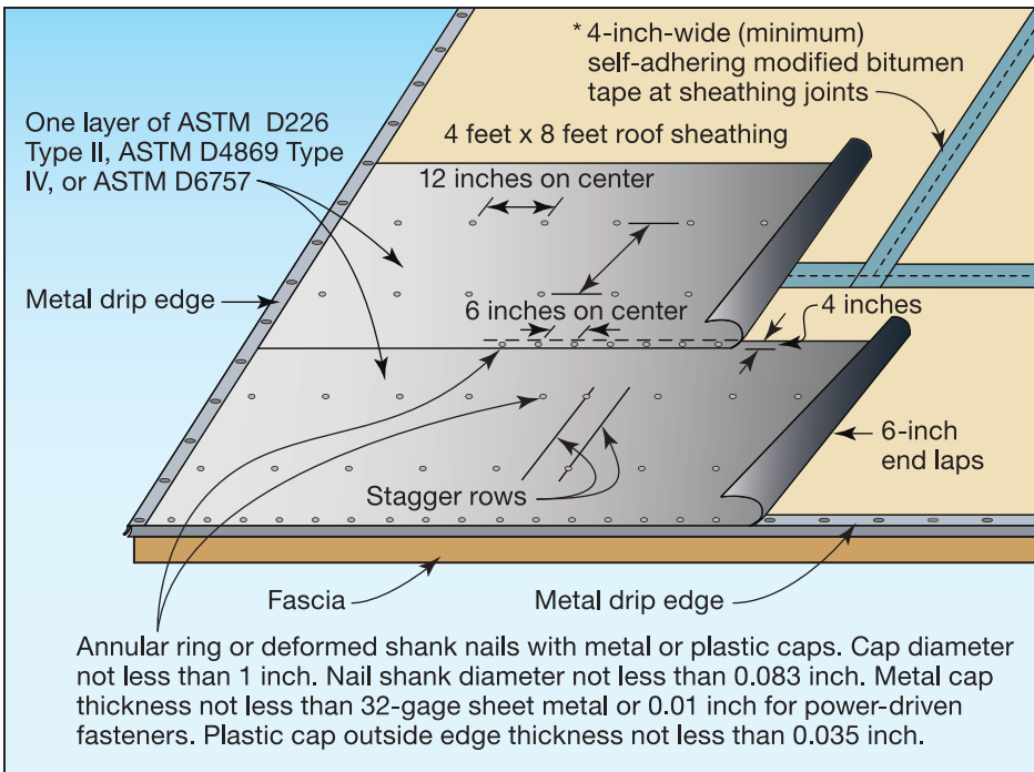
Figure 6: Option 2 for installing a sealed roof deck to reduce water infiltration through the roof
