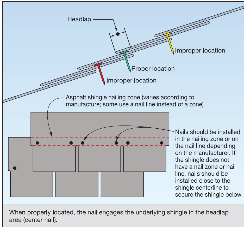
Figure 2: Proper and improper locations of shingle fasteners
