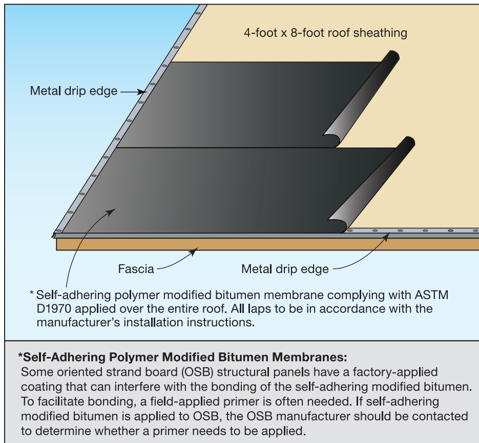
Figure 5: Option 1 for installing a sealed roof deck to reduce water infiltration through the roof
