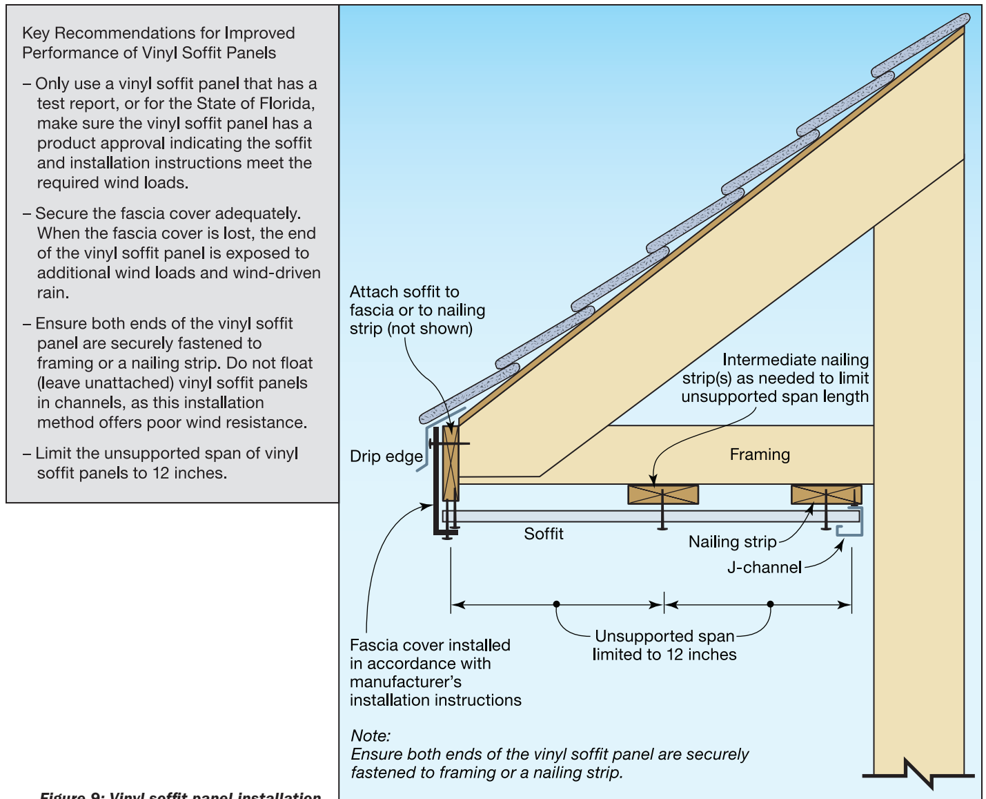
Figure 9: Vinyl soffit panel installation
