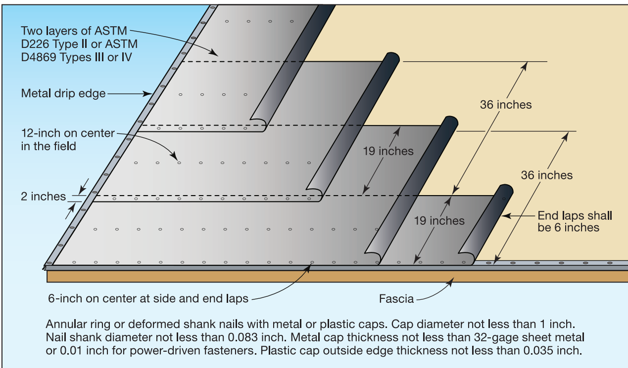
Figure 7: Option 3 for installing a sealed roof deck to reduce water infiltration through the roof
