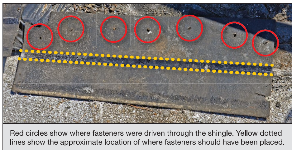
Figure 3: Incorrect location of fasteners in an asphalt shingle
